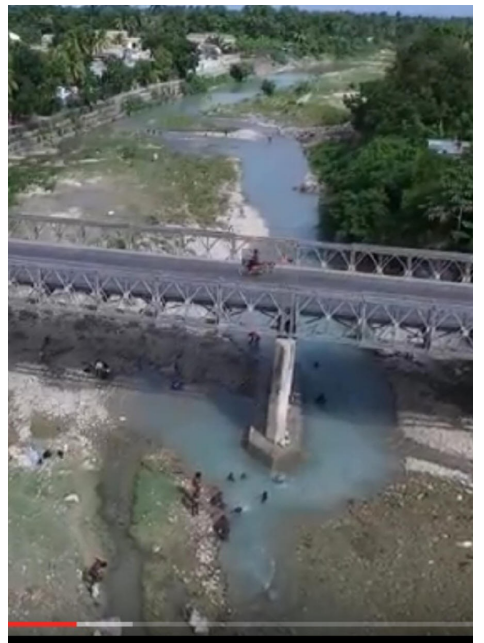
Figure 16 "Drone" Bridge that washed-out.
